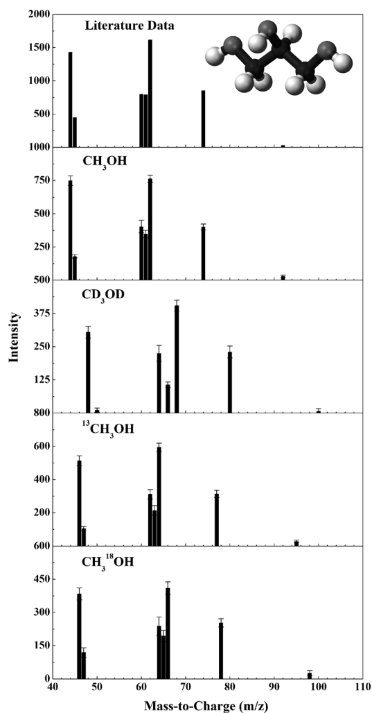
Figure 4. Integrated ion signal at distinct mass-to-charge ratios relevant to fragment and parent ions associated with glycerol formation ( \text{C}_2\text{H}_4\text{O}^+ , \text{C}_2\text{H}_5\text{O}^+ , \text{C}_2\text{H}_4\text{O}_2^+ , \text{C}_2\text{H}_5\text{O}_2^+ , \text{C}_2\text{H}_6\text{O}_2^+ , \text{C}_3\text{H}_6\text{O}_2^+ , \text{C}_3\text{H}_8\text{O}_3^+ ) together with their isotopically substituted counterparts in irradiated \text{CH}_3\text{OH} , \text{CD}_3\text{OD} , ^{13}\text{CH}_3\text{OH} , and \text{CH}_3^{18}\text{OH} ices obtained at a photo-ionization energy of 10.49 eV. The top graph presents the literature data extracted from ReTOF spectra of glycerol recorded with a photo-ionization energy of (10.50 \pm 0.02) eV. [22] The insert portrays the molecular structure of the glycerol molecule which carbon (black), hydrogen (light gray), and oxygen atoms (dark gray).
